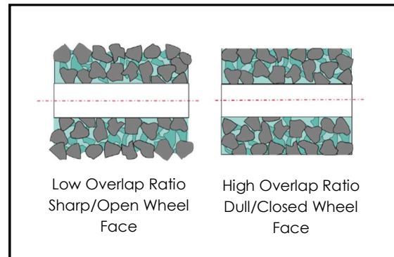
Figure 4 – Sharp and Dull Wheel Face
